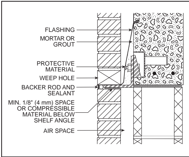
Shelf Angle Detail FIG. 8
