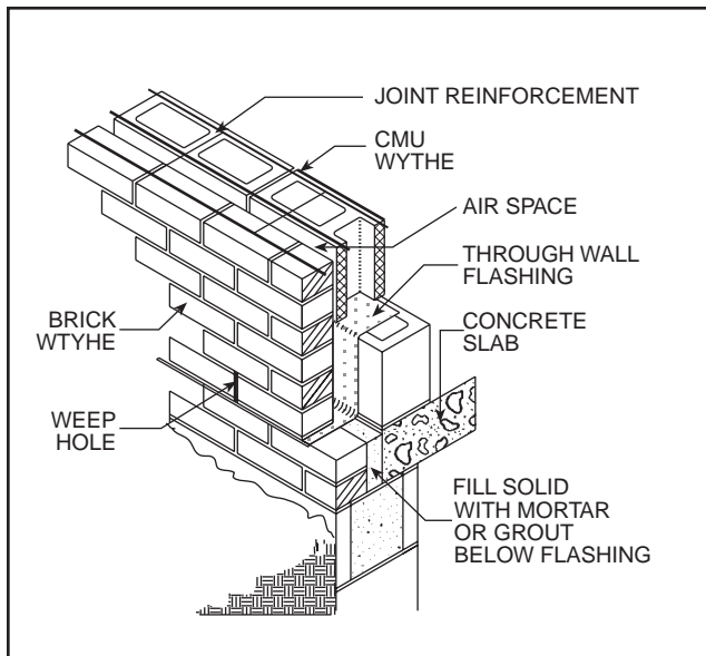
Basement Detail FIG. 5
