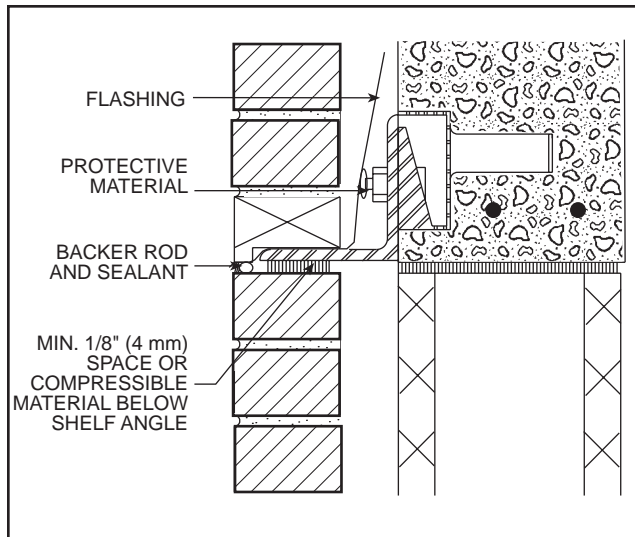
Lipped Brick Detail FIG. 17
