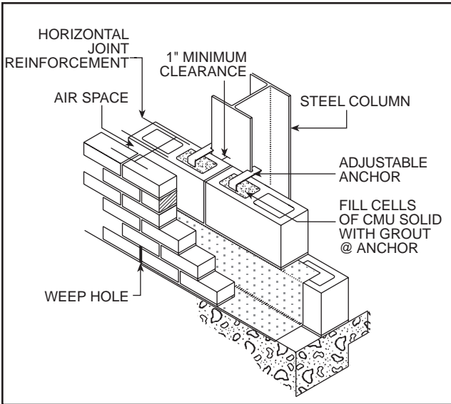
Anchorage to Steel Column (From Masonry and Steel Detailing Handbook , W. Laska) (Fireproofing omitted for clarity) FIG. 19
