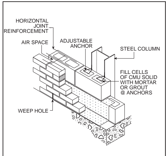
Anchorage to Steel Column (From Masonry and Steel Detailing Handbook , W. Laska) (Fireproofing omitted for clarity) FIG. 18
