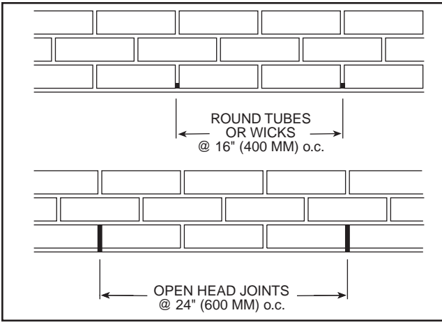
Spacing of Weep Holes FIG. 2
