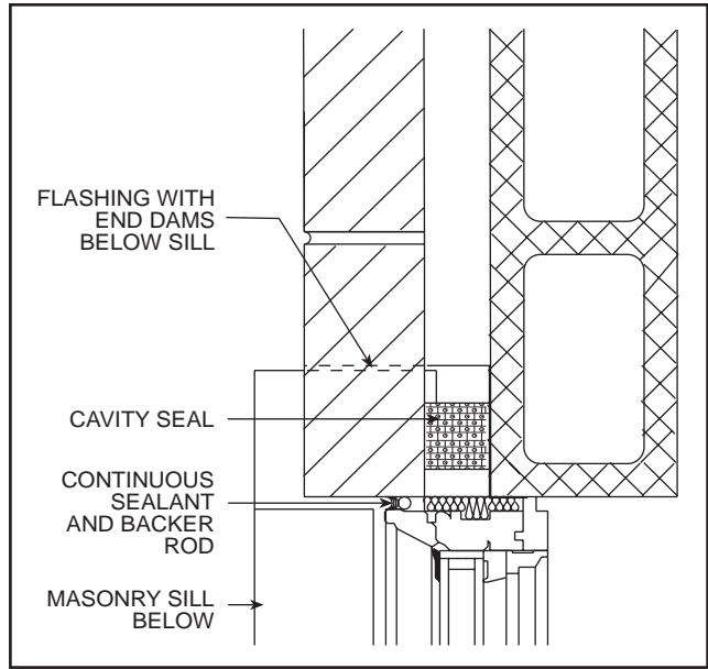
Window Jamb Detail with Cavity Seal FIG. 10
