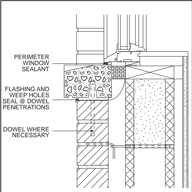
Window Sill Detail FIG. 13
