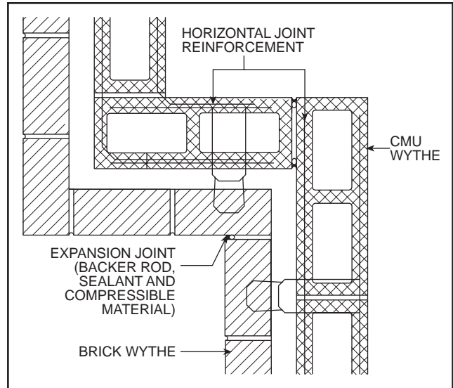
Vertical Expansion Joint at Interior Corner FIG. 15
