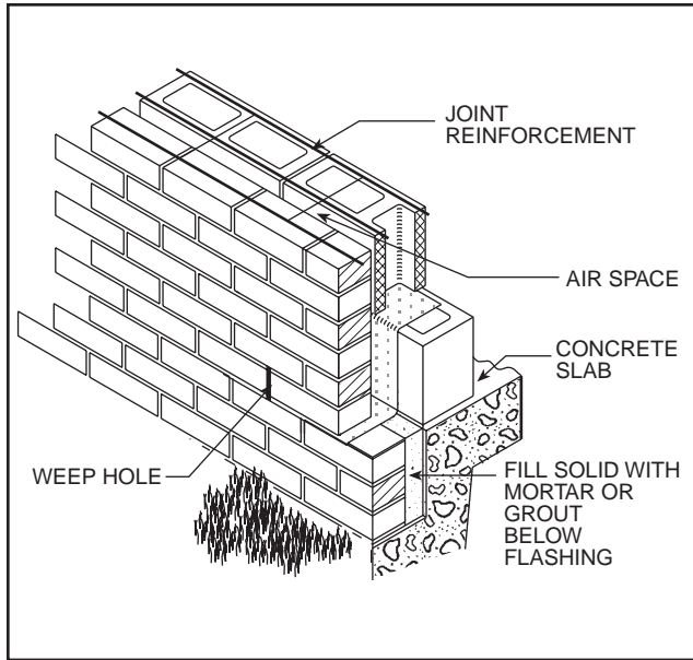
Foundation Detail FIG. 4
