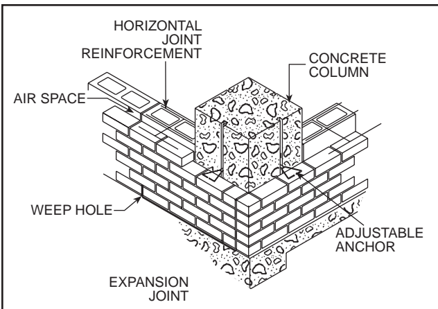
Anchorage to Concrete Column FIG. 20
