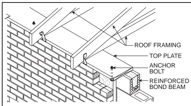
Wood Roof Framing Detail FIG. 24
