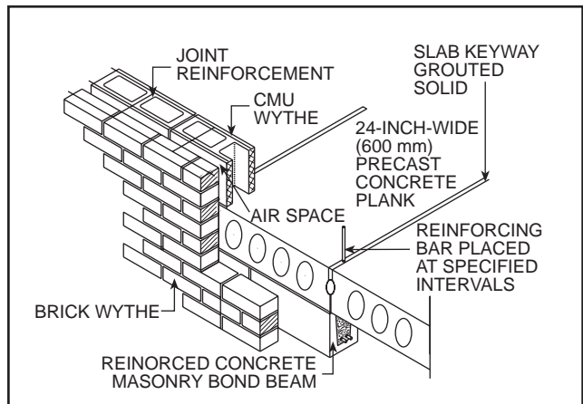
Steel reinforced Concrete Plank Bearing FIG. 22
