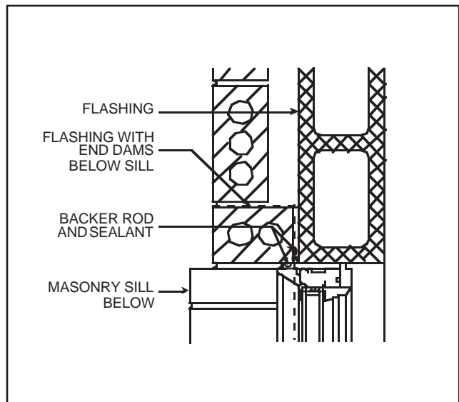
Window Jamb Detail FIG. 11
