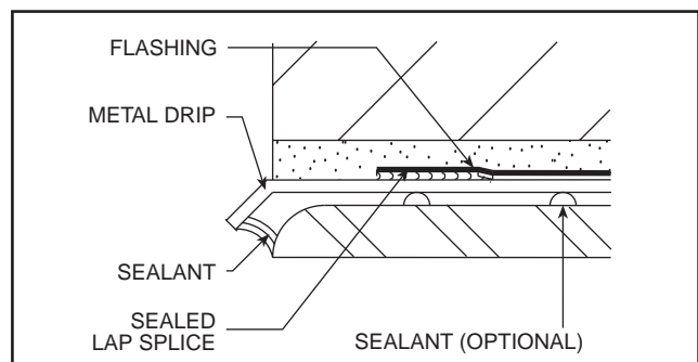
Flashing with Metal Drip Edge FIG. 1
