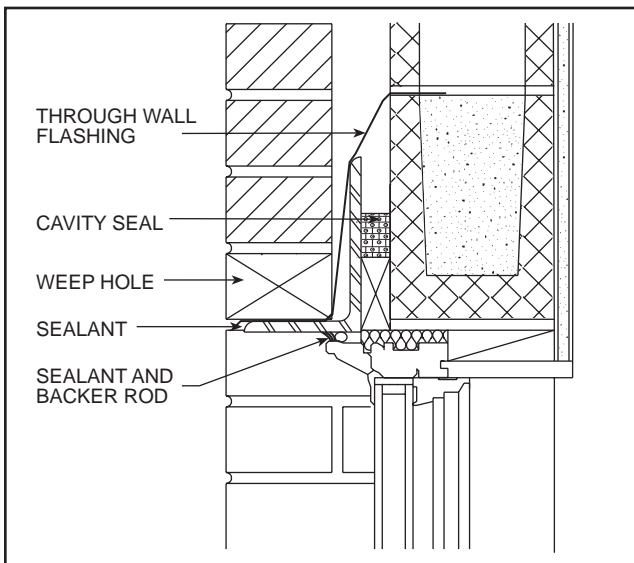
Window Head Detail and Cavity Seal FIG. 9
