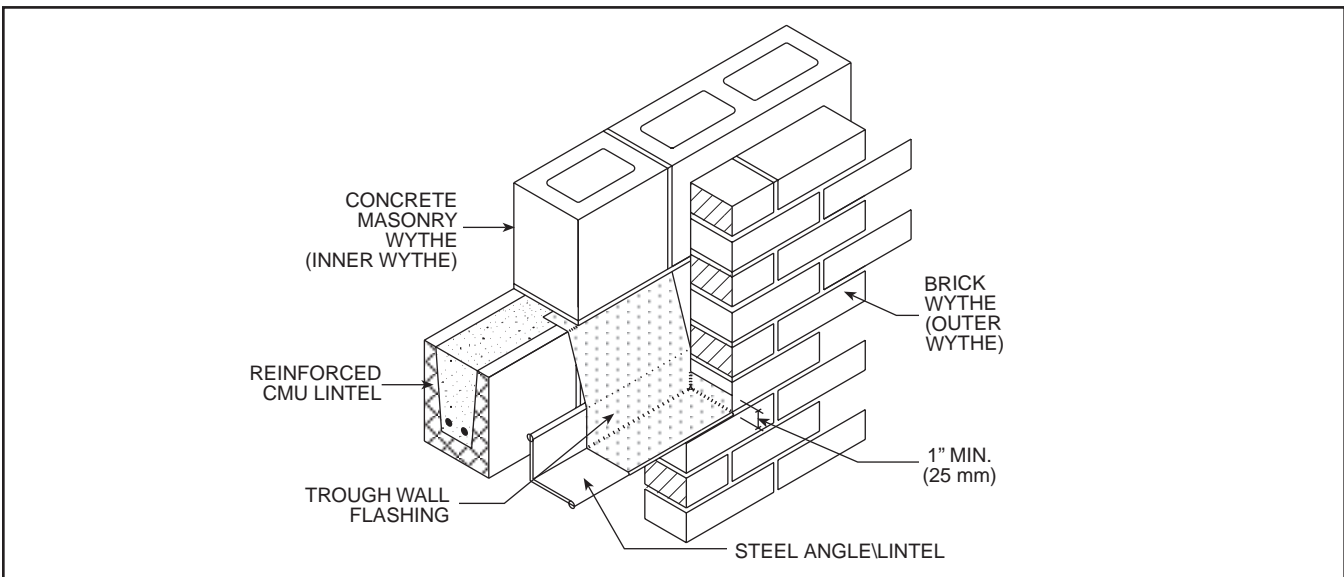
End Dam FIG. 3
