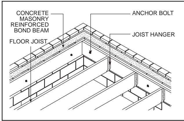
Wood Floor Joist Connection Detail FIG. 23
