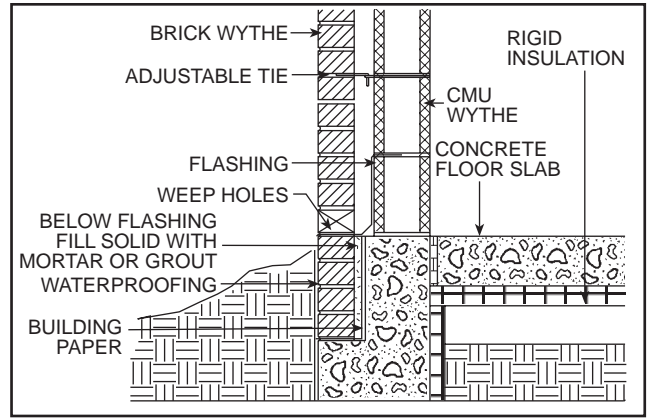
Foundation Detail FIG. 25
