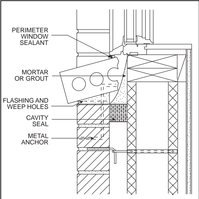
Window Sill Detail FIG. 12
