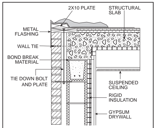
Concrete Roof Slab Detail FIG. 26
