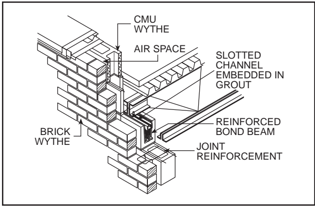
Steel Joist Bearing (From Masonry and Steel Detailing Handbook , W. Laska) FIG. 21
