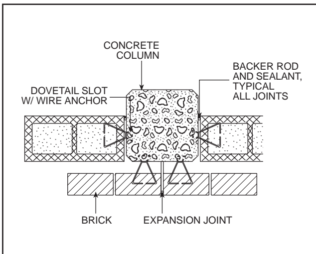
Vertical Expansion Joint FIG. 14
