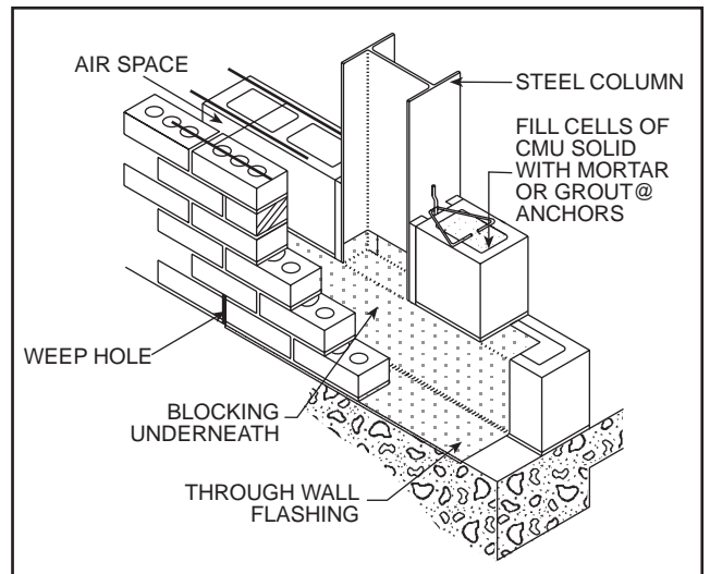
Flashing at Steel Column (From Masonry and Steel Detailing Handbook, W. Laska ) FIG. 7
